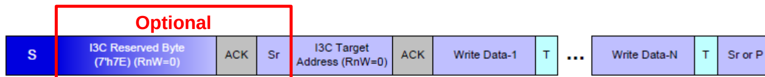
I3C Private Write Transfer Initiated with START Condition
